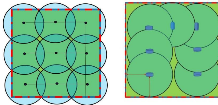
(a) Traditional (b) Enhanced Fig.6 Traditional vs. Enhanced sprinklers
