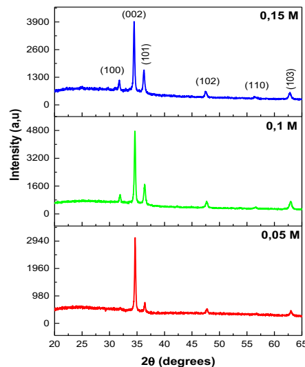
Fig 1: XRD patterns of the deposited ZnO thin films for different molarities.
