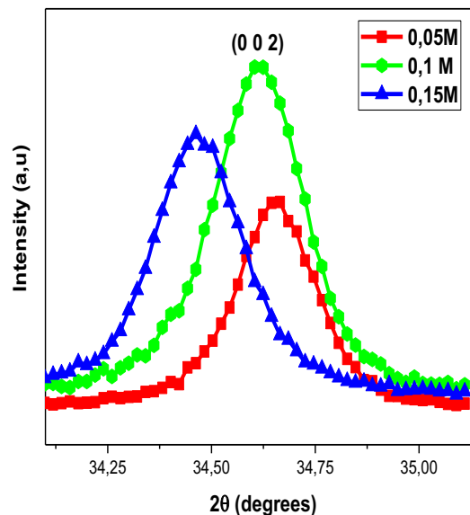
Fig.2: (002) peak position of the ZnO films for different molarities.
