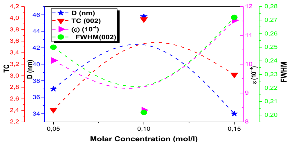
Fig 4: the average crystallite size (D), texture coefficient (TC), micro-strain ( \varepsilon ) and FWHM Of ZnO thin films prepared for different molarities.
