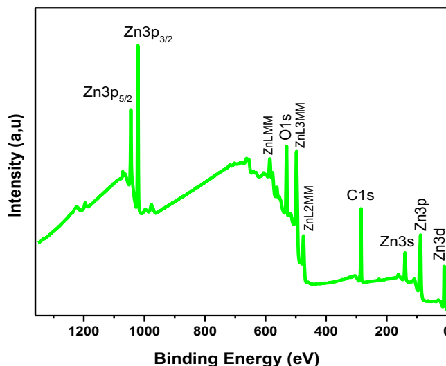
Fig. 3: XPS survey spectrum of ZnO thin films prepared with molarity 0.1M.
