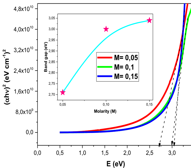
Fig 6: Variation of (\alpha h\nu)^2 against photon energy ( h\nu ).
