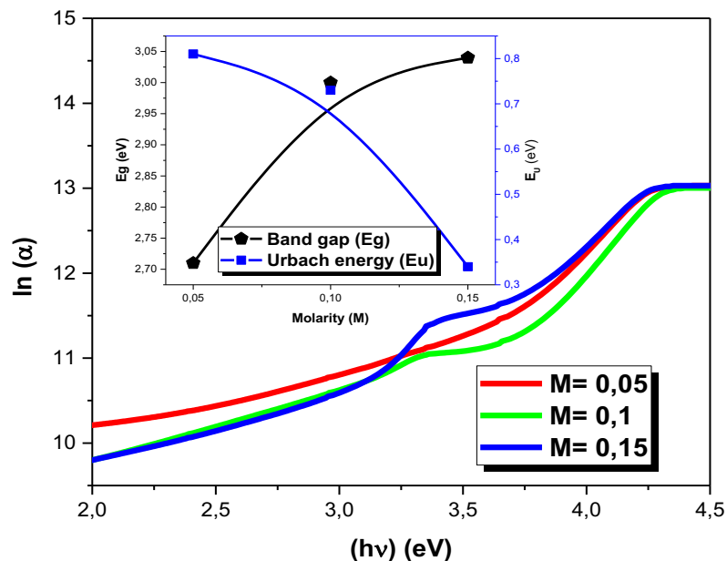
Fig 7: Variation of Urbach energy and optical Band gap of samples against molarity.
