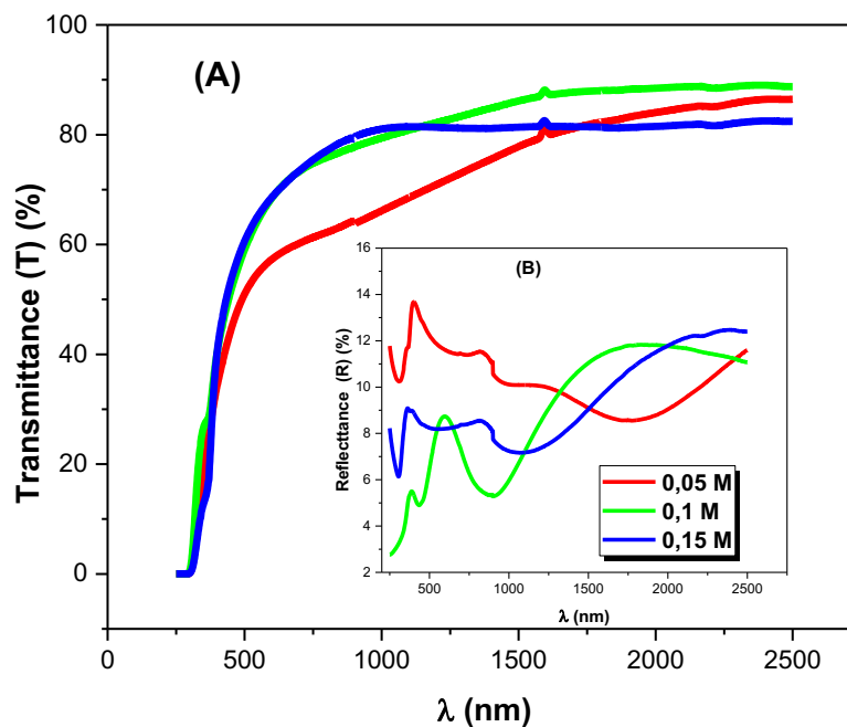
Fig 5 (A, B): Optical transmittance and reflectance of ZnO thin films for different molarities.
