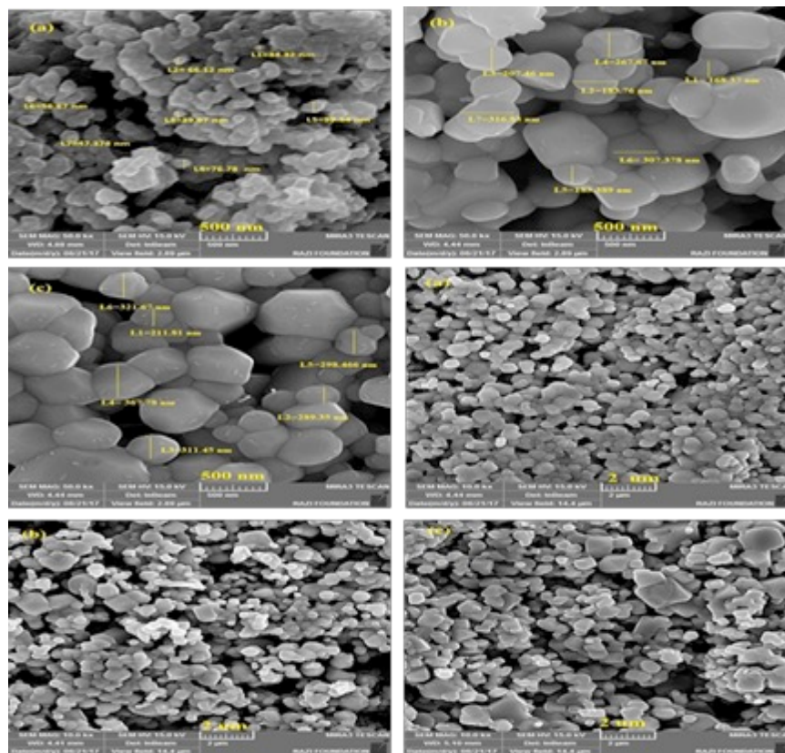
Fig.6: FES E M micrograph of Ferroelectric Ba_{0.7}Sr_{0.3}TiO_3 sintered at various temperatures (a) 900 °C, (b) 1000 °C, (c) 1100 °C.
