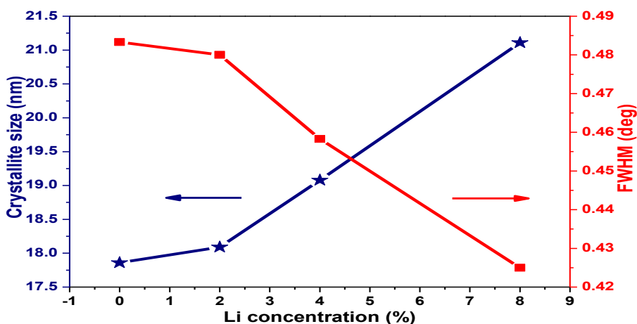
Fig.2: The variations of lattice constant and crystallite size of undoped and Li dopedNiO thin films.
