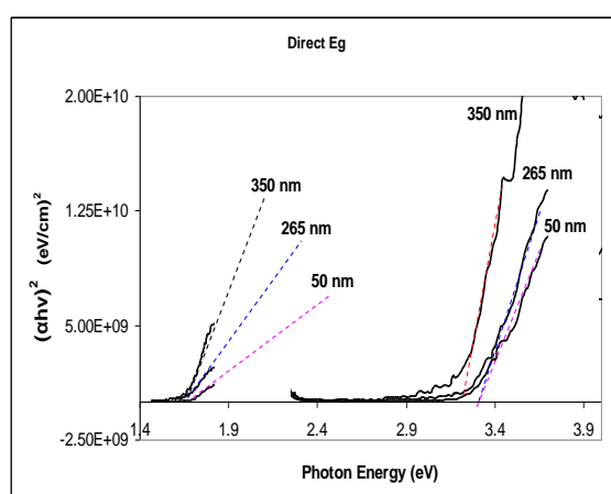
Fig.4 Direct energy band gaps for UV-Visible spectra
