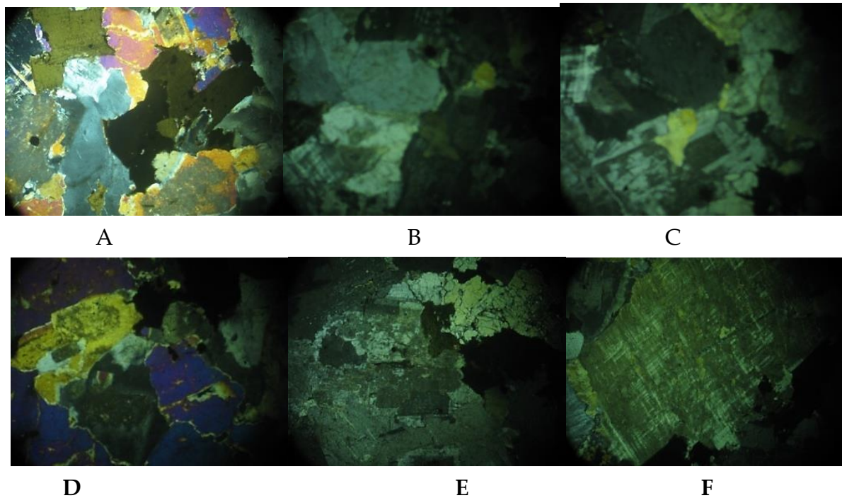
[FIGURE 3]: Petrographic study of granite sample by PLM, x. 40: A.)Granite samples appear pink, coarse-grained and large, quartz and feldspar are the main component of granite; B). quartz crystals appear;C). gypsum stains as one of the products of damage as a result of the changes that occurred, and the transformation of biotite mineral to kaolin;D). increase in pressures due to the swelling of clay minerals; E & F). Some of the fractures that are products of damage.
