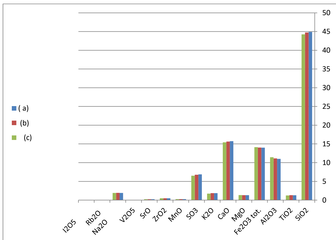
[FIGURE 6]: Main Constituents Wt%.
