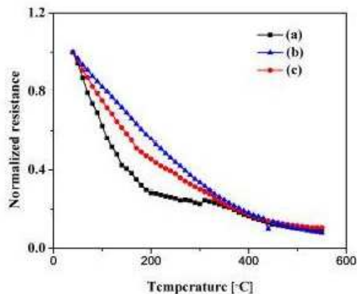
Figure 8: Normalized resistance versus temperature for 3C-SiC thin films deposited at a pressures of (a) 1.5, (b) 2.5 and (c) 2.7 mbar
