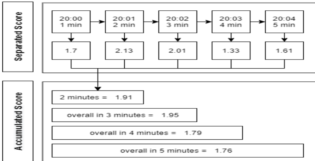
Figure 5-2: calculating the separated score and accumulated score in the timeframe.
