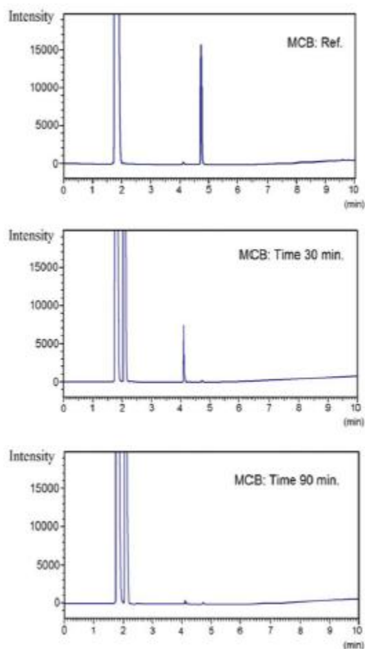
Figure 11: The GC analysis of MCB degradation by TiO 2 -TX100 - SiO 2 films under UV light in different times (0, 30 & 90 min).
