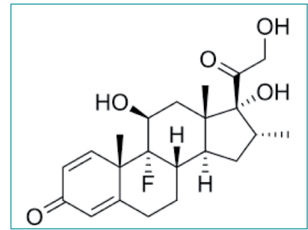
Fig. 1: Dexamethasone structure.
