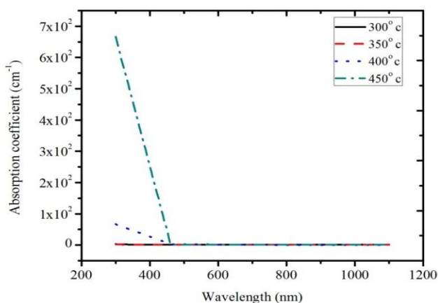
Figure 6: Response of Absorption spectra of Ti doped Indium Oxide thin films for various substrate temperatures
