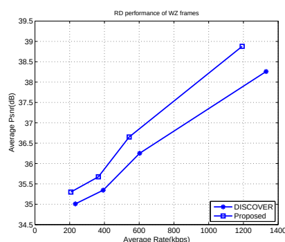
Figure 4: Coastguard.
