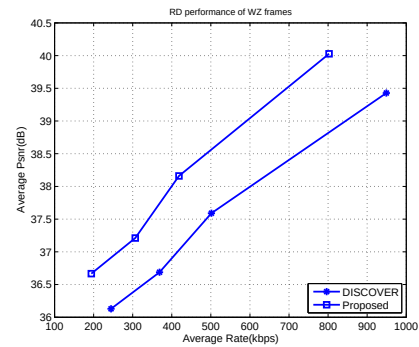
Figure 3: Foreman.
