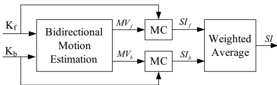
Figure 2: Motion Compensated Interpolation.
