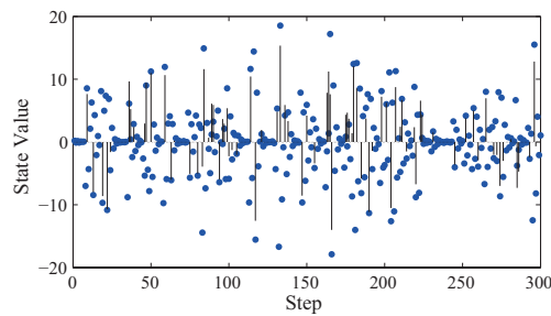
Figure 6 PSO-PF estimate
