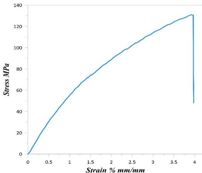
Fig. 16: Stress-strain behavior of (0)8 NYRP laminate under flexure test.
