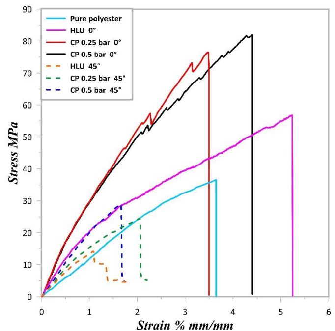
Figure 11: Stress-strain behavior of different NYRP laminates under tensile test.
