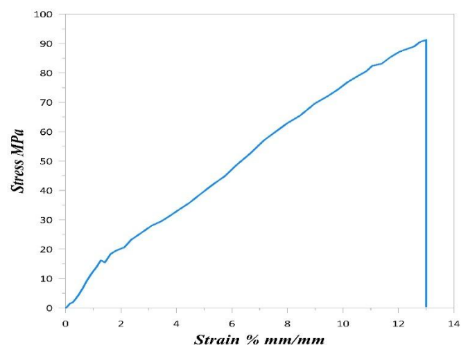
Fig. 15: Stress-strain behavior of (0)8 NYRP laminate under tensile test.
