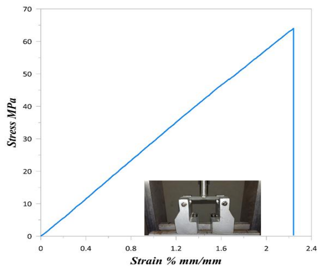
Fig. 9: Stress-strain behavior under flexure for pure polyester.
