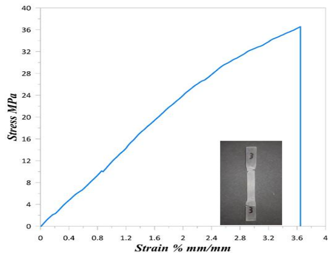
Fig. 8: Stress-strain behavior under tension for pure polyester.
