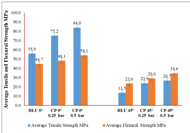
a) Average tensile and flexural strengths
