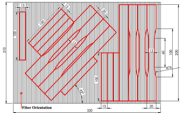
Fig. 6: Schematic cutting patterns of preparing NYRP composite specimens for tensile and flexure tests.
