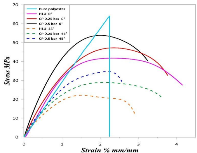
Fig. 14: Stress-strain behavior of different NYRP laminates under flexure test.
