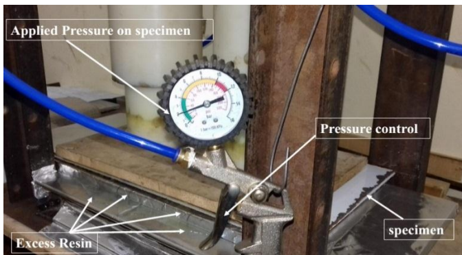
Fig. 3: The configuration of the compression machine.
