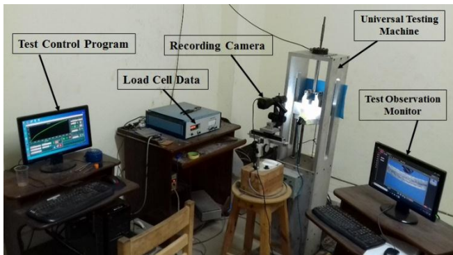
Fig. 4: Universal Testing Machine in Polymer Lab.
