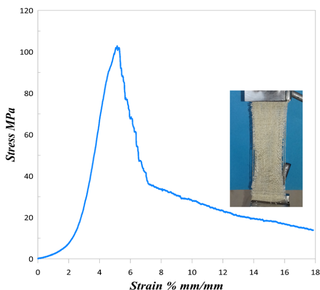
Fig. 7: Stress-strain behavior in tensile test of non-impregnated flax fabric.
