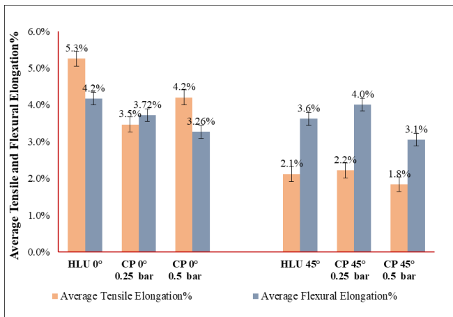
c) Average tensile and flexural elongation %
