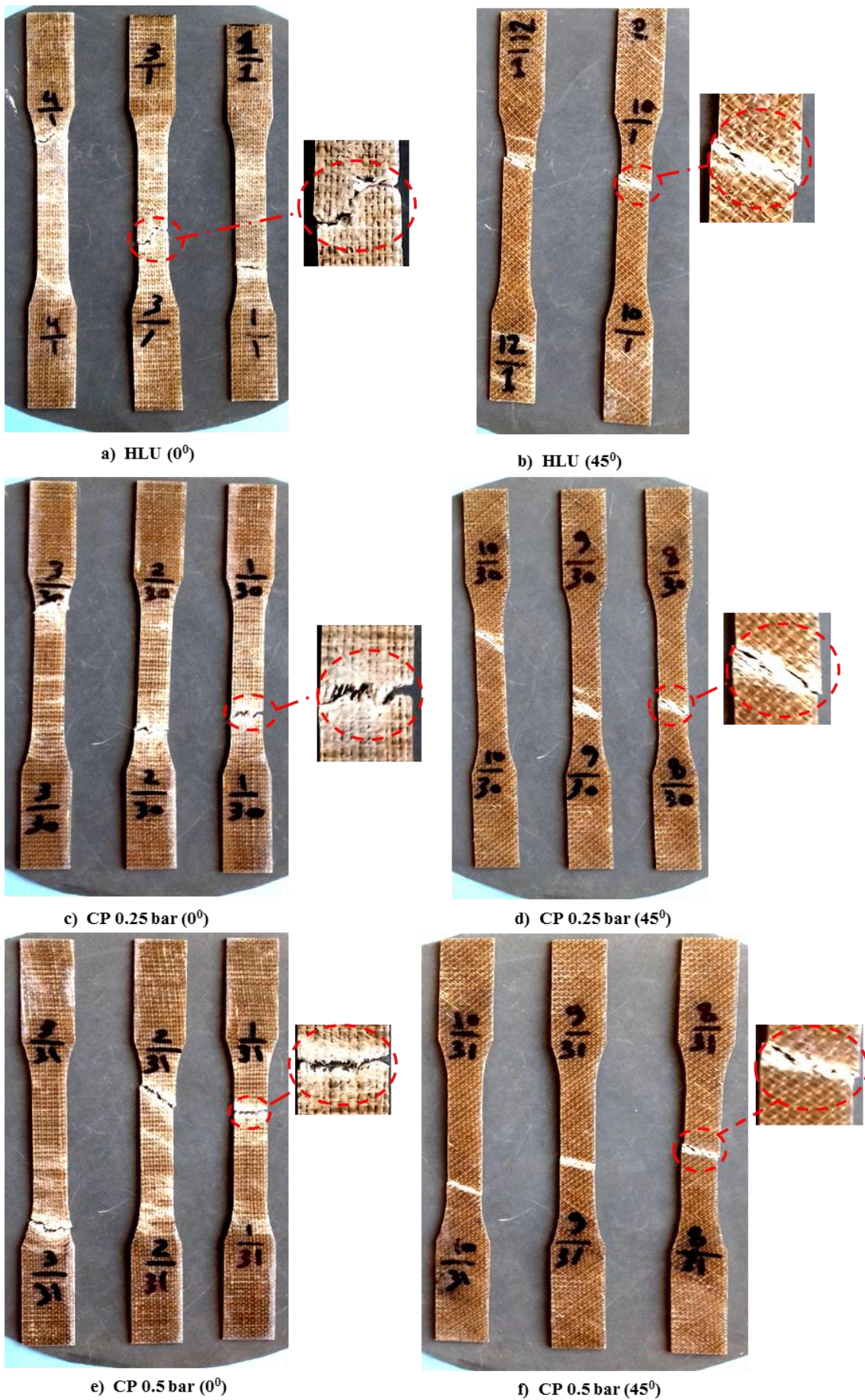
Fig. 13: Common modes of failure observed for different NYRP laminates under tensile test.
