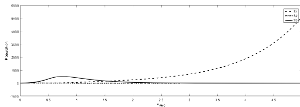
Fig. 3: Time series shows the behavior of three species.
