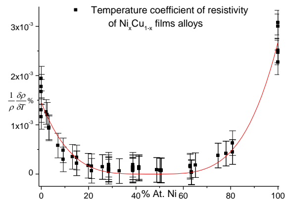
Fig.12b: Variation of the temperature coefficient of resistivity according to the nickel content in \text{Ni}_x\text{Cu}_{1-x} alloy films.
