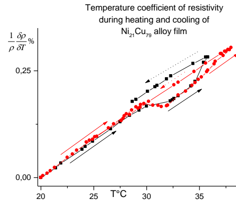
Fig.12a: Variation of the temperature coefficient of resistivity, during heating and cooling, near the ambient temperature in \text{Ni}_{21}\text{Cu}_{79} alloy films.
