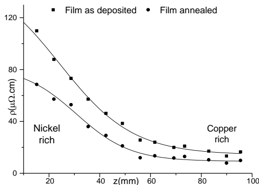
Fig.11b: Effect of the annealing on the resistivity of \text{Ni}_x\text{Cu}_{1-x} alloy films deposited on \alpha -alumina substrate.
