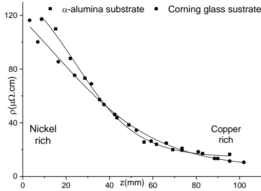
Fig.11a: Influence of the substrate on the resistivity of \text{Ni}_x\text{Cu}_{1-x} alloy films as deposited.
