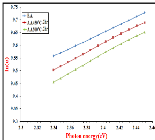
Fig. (6): Urbach energy of ZnFe 2 O 4 films before and after annealing.
