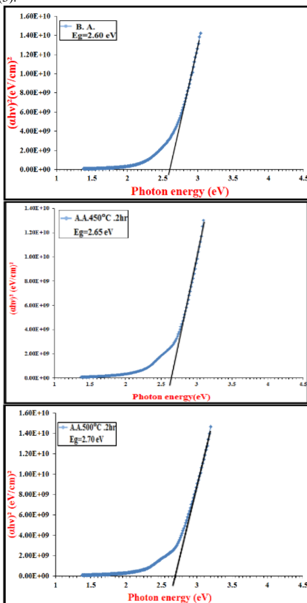
Fig. (5): Energy gap of ZnFe 2 O 4 films before and after annealing.
