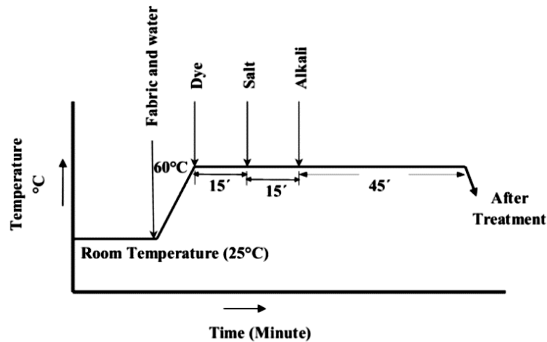
Figure 1. Reactive dyeing curve.
