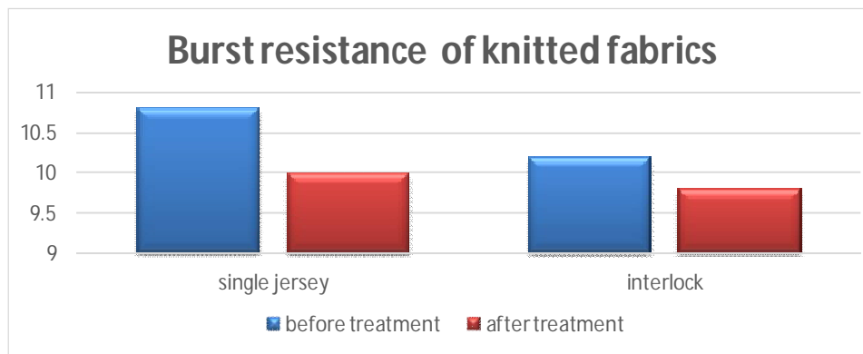
Figure 2. Effects of cellulase enzyme on burst resistance of different knitted T-shirts fabrics.
