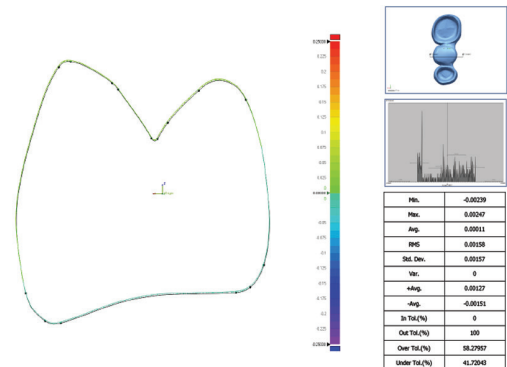
Figure (3): Compare 3 of remote design (T/O) to host design (TD)
