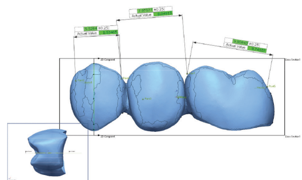
Figure (5): Linear Measurements of Remote Design (T/O) to Host Design (TD)
