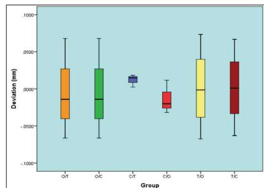
Figure (7): Box plot representing median and range values for trueness of the different designs in cross section 1
