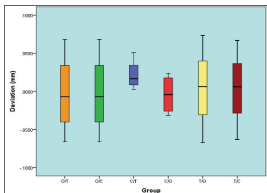
Figure (6): Box plot representing median and range values for trueness of the different designs in 3D
