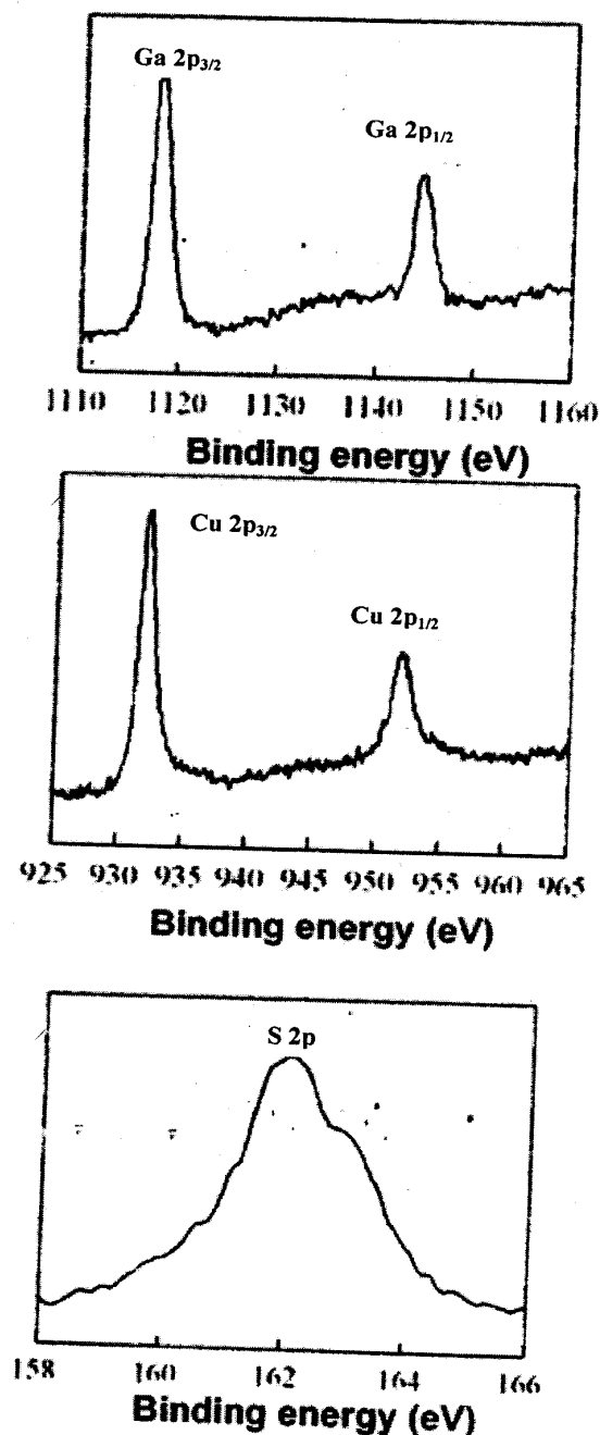
Fig. 4 XPS spectra of \text{CuGaS}_2 films deposited at 80°C electrolyte temperature.
