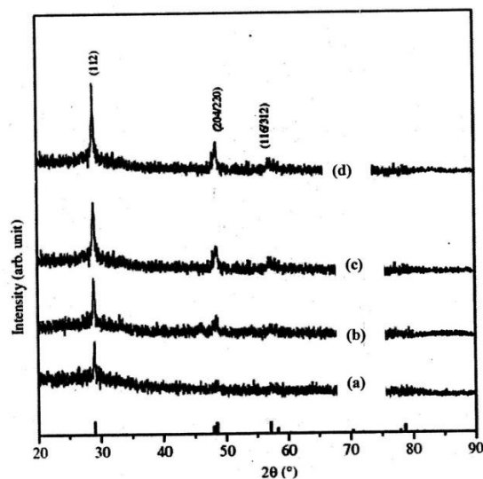
Fig. 2 X-ray diffraction pattern of \text{CuGaS}_2 films deposited at different electrolyte temperature (a) 30^\circ\text{C} (b) 50^\circ\text{C} (c) 70^\circ\text{C} (d) 80^\circ\text{C} .
