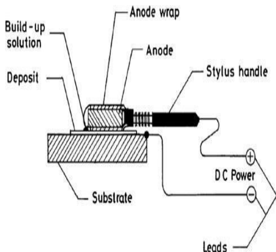
Fig. 1 Schematic of the brush plating system
