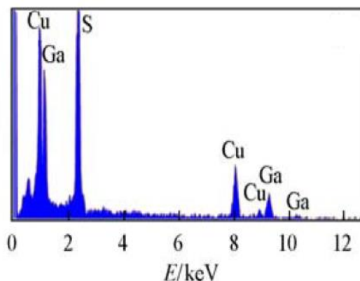
Fig. 3 EDS spectrum of CuGaS 2 films deposited at 80°C electrolyte temperature
