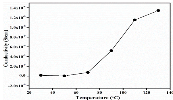
Fig 9. Conductivity of CdO nanoparticle.
