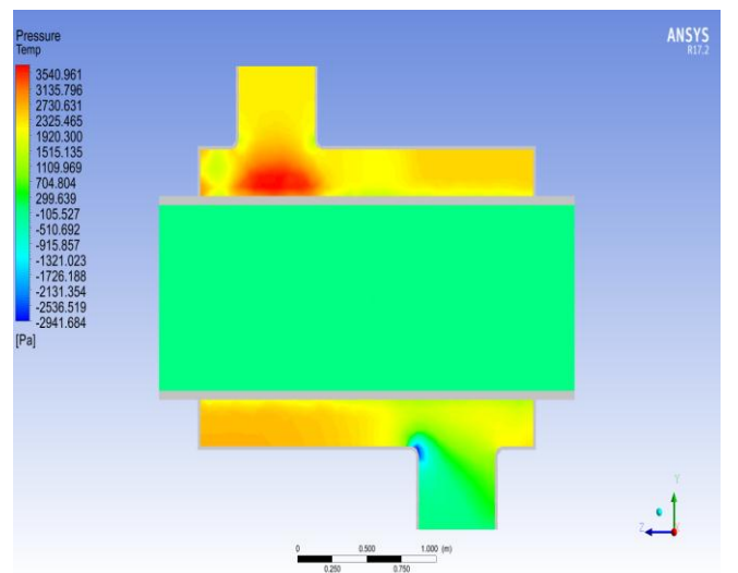
Figure 17. Pressure distribution on a plane for the shell & tube (Hot & cold fluid) in shell and heat exchanger for the first case.
