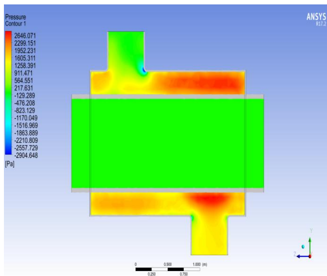
Figure 28. Pressure distribution on a plane for the shell & tube (Hot & cold fluid) in shell and heat exchanger for the second case
