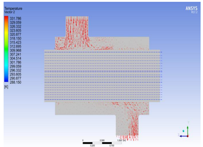
Figure 16 Direction of Temperature on a plane for the shell & tube (Hot & cold fluid) in shell and heat exchanger for the first case.
