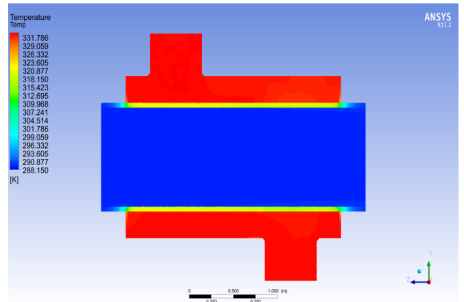
Figure 15 Temperature distribution on a plane for the shell & tube (Hot & cold fluid) in shell and heat exchanger for the first case.
