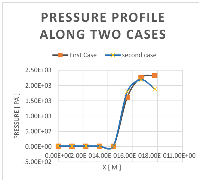
Figure 32. Comparison for pressure profile along Heat exchanger for the two cases.
