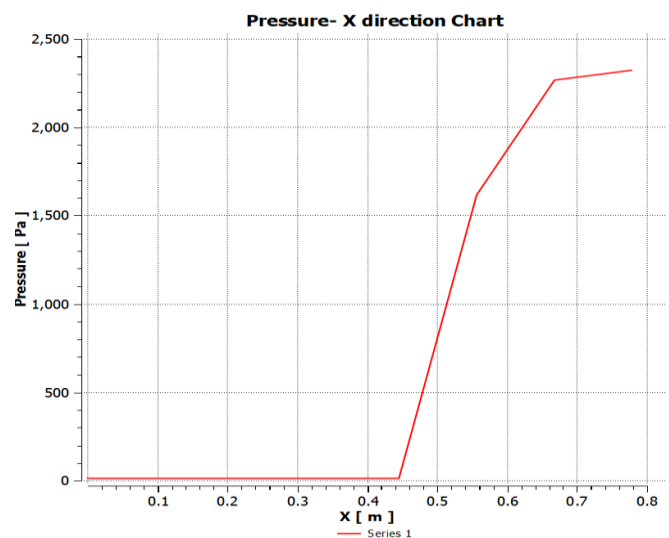
Figure 10. Pressure Chart
