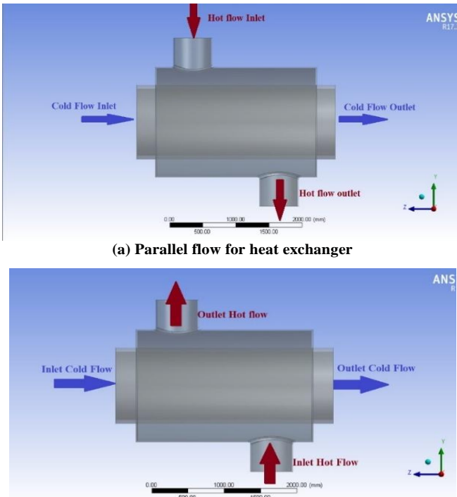
Figure 5. (a&b) Flow Direction for shell and tube heat exchanger one tube & one pass
