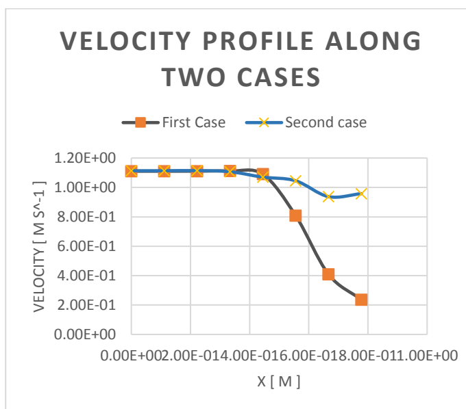
Figure 33. Comparison for Velocity profile along Heat exchanger for the two cases.
