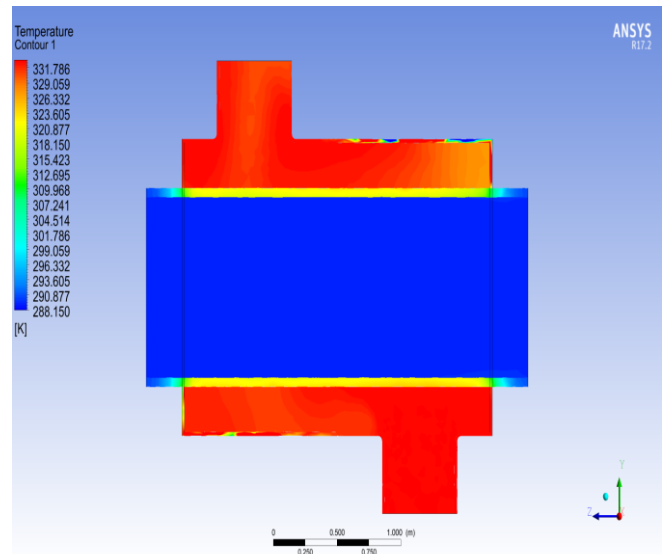
Figure 26. Temperature distribution on a plane for the shell & tube (Hot & cold fluid) in shell and heat exchanger for the fourth case.
