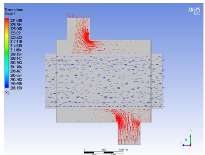
Figure 27. Direction of Tempe on a plane for the shell & tube (Hot & cold fluid) in shell and heat exchanger for the second case.
