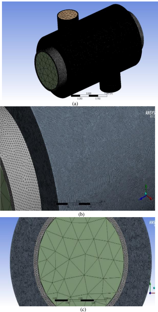
Figure 7. (a),(b) &(c) Different views for Coarse mesh for shell and tube heat exchange
