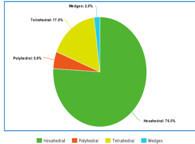
Figure 8. Mesh Composition
