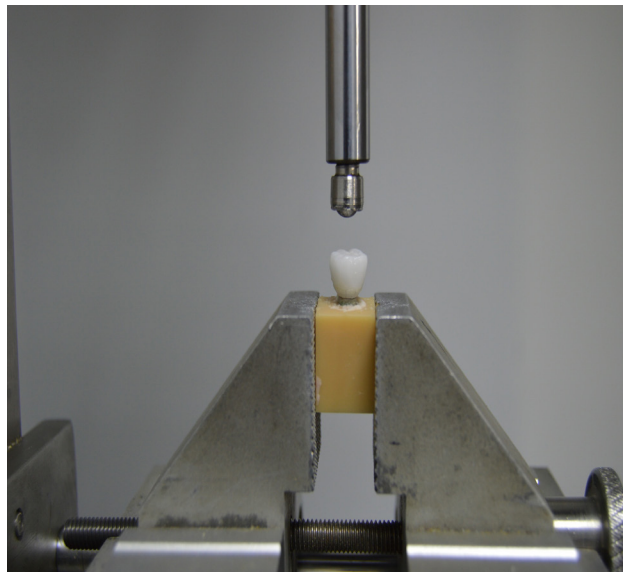
Fig 2. Specimen placed on the YLE® universal testing machine
