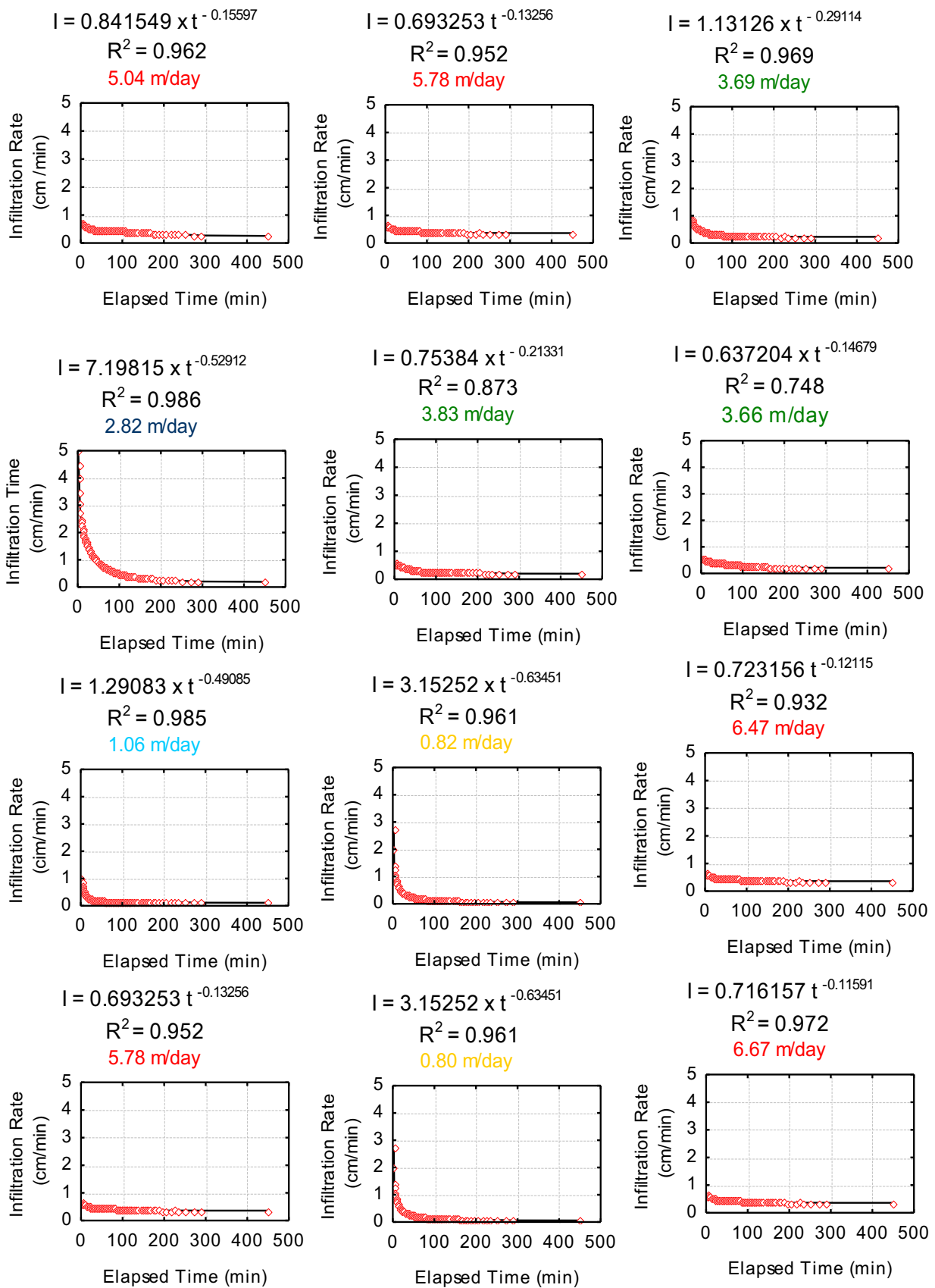
Figure 13. Infiltration characteristics (infiltration rate) of the soil profiles.
