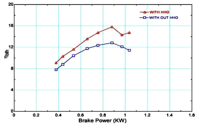
Fig. 3. Thermal Efficiency and brake power [36]
