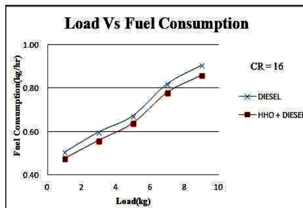
Fig. 5. Variation of fuel consumption with load [57]
