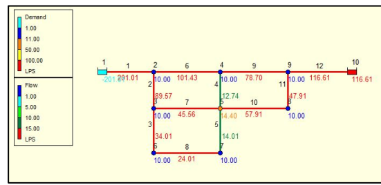
Fig. 6: Water distribution network with one leak and 8 demand sources (leak on node).
