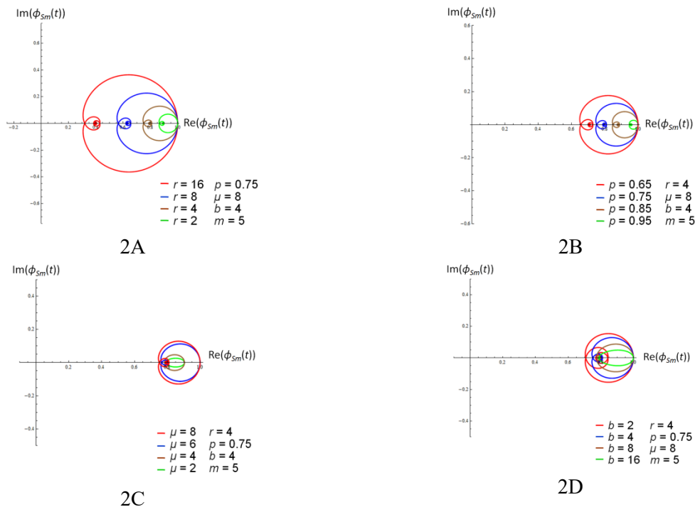
Fig. 2: Parametric curves of characteristic function from m -division of compound negative binomial distribution as the sum of Laplace distribution with various parameters.
