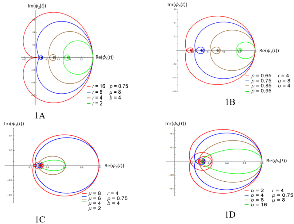
Fig.1: Parametric curves of characteristic function from compound negative binomial distribution as the sum of Laplace distribution with various parameters.
