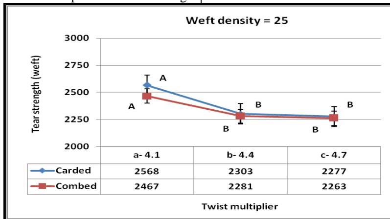
Fig. (4): The effect of twist multiplier on fabric weft tearing strength for two spinning systems (carded and combed) under weft density (25).
