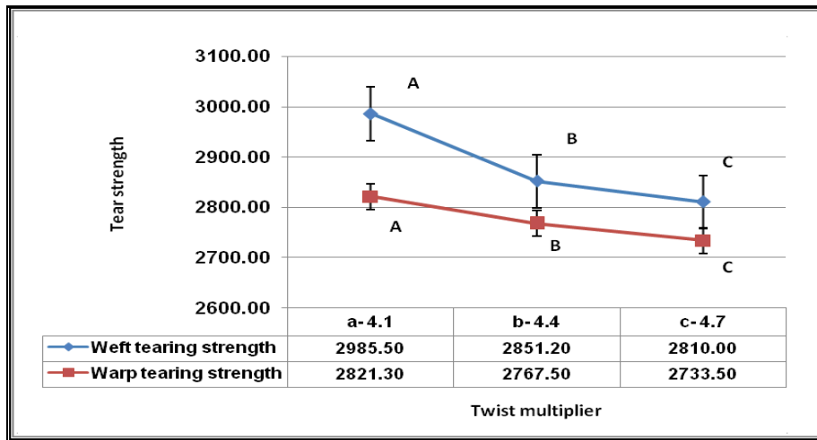
Fig. (1): The effect of twist multiplier on weft and warp tearing strengths overall studied factors.
