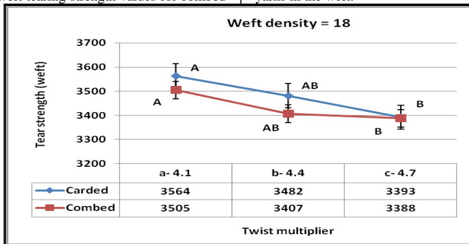
Fig. (2): The effect of twist multiplier on weft tearing strength for two spinning systems (carded and combed) under weft density (18).
