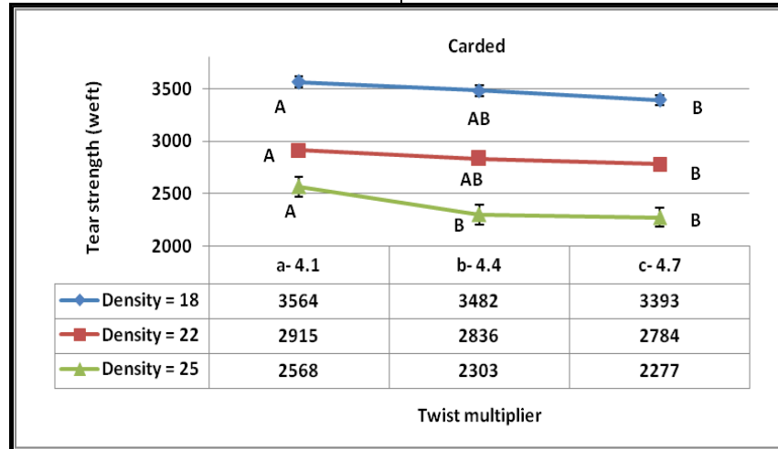
Fig. (5): The effect of twist multiplier on weft tearing strength for three weft densities (18, 22 and 25) using carded spun yarns.
