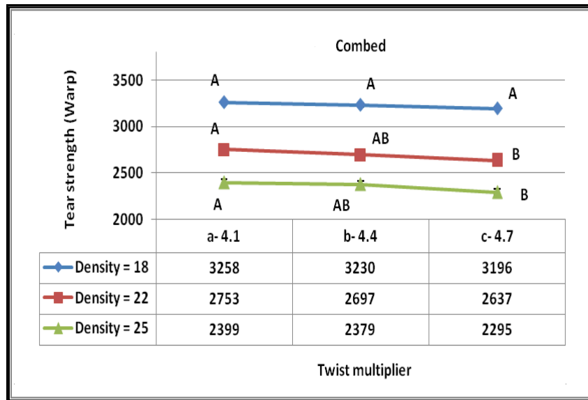
Fig. (11): The effect of twist multiplier on warp tearing strength for three weft densities (18, 22 and 25) using combed spun yarns.
