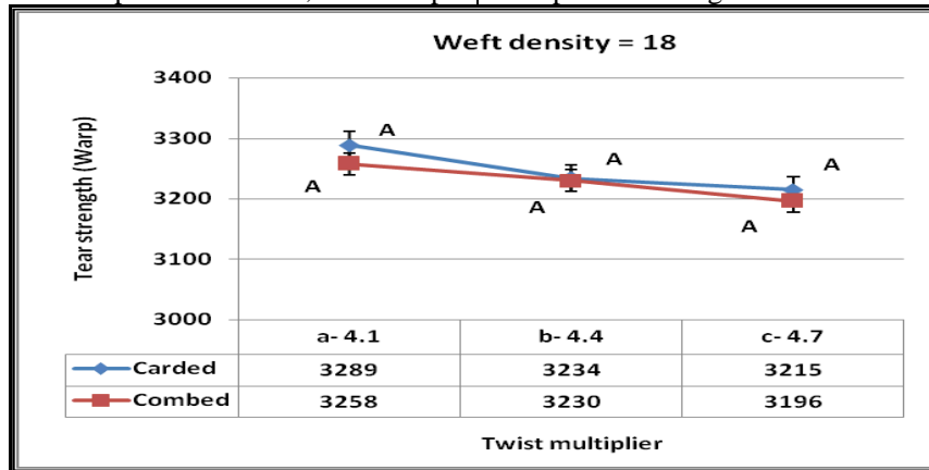
Fig. (7): The effect of twist multiplier on warp tearing strength for two spinning systems (carded and combed) under weft density (18).
