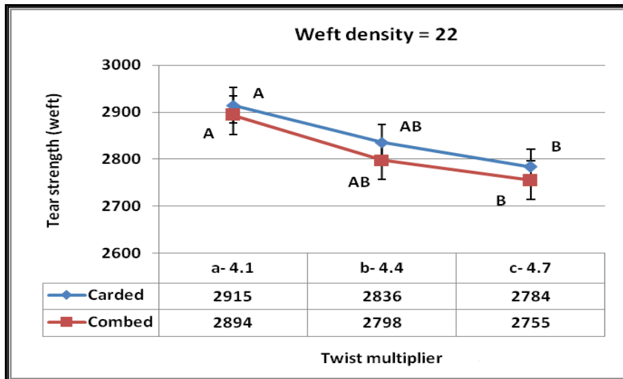
Fig. (3): The effect of twist multiplier on fabric weft tearing strength for two spinning systems (carded and combed) under weft density (22).
