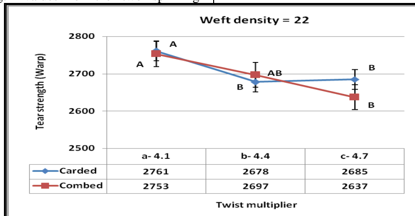
Fig. (8): The effect of twist multiplier on warp tearing strength for two spinning systems (carded and combed) under weft density (22).
