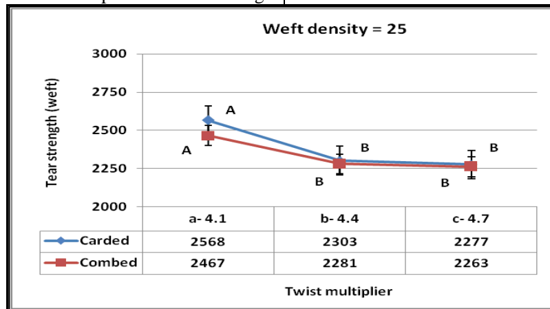
Fig. (4): The effect of twist multiplier on fabric weft tearing strength for two spinning systems (carded and combed) under weft density (25).
