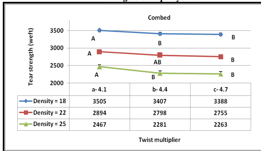
Fig. (6): The effect of twist multiplier on weft tearing strength for three weft densities (18, 22 and 25) using combed spun yarns.
