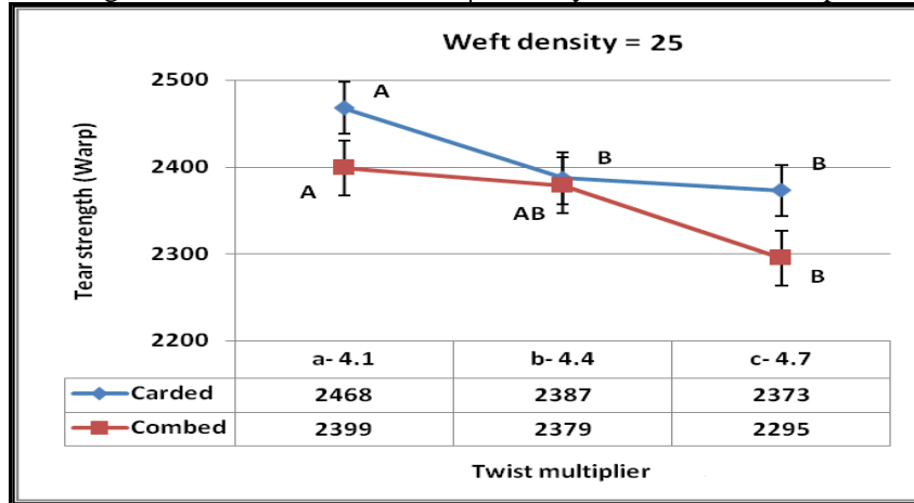
Fig. (9): The effect of twist multiplier on warp tearing strength for two spinning systems (carded and combed) under weft density (25).
