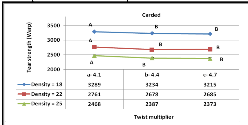
Fig. (10): The effect of twist multiplier on warp tearing strength for three weft densities (18, 22 and 25) using carded spun yarns
