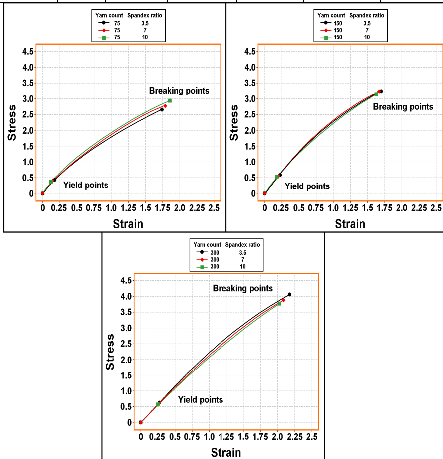
Fig. (5): Stress-strain curves of spandex/polyester spun yarn as affected by the interaction effect between yarn count and spandex ratio.
