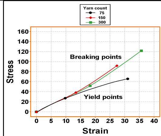
Fig. (8): Stress-strain curves of spandex/polyester woven fabrics as affected by yarn count.
