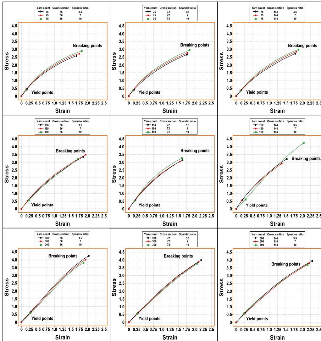
Fig. (7): Stress-strain curves of spandex/polyester spun yarn as affected by the interaction effect among yarn count, cross section and spandex ratio.
