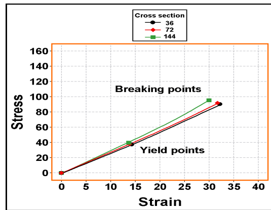
Fig. (9): Stress-strain curves of spandex/polyester woven fabrics as affected by cross section.
