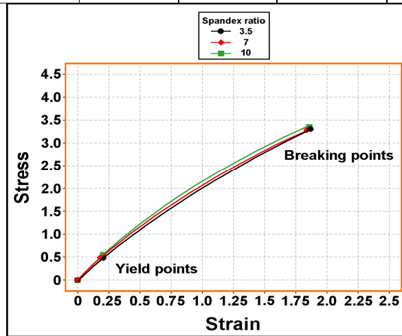
Fig. (3): Stress-strain curves of spandex/polyester spun yarn as affected by spandex ratio.
