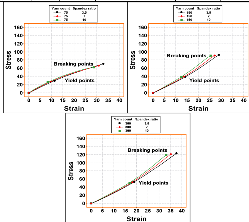
Fig. (12): Stress-strain curves of spandex/polyester woven fabrics as affected by the interaction effect between yarn count and spandex ratio.
