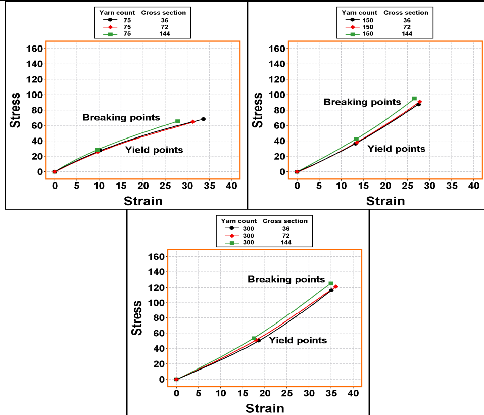
Fig. (11): Stress-strain curves of spandex/polyester woven fabrics as affected by the interaction effect between yarn count and cross section.
