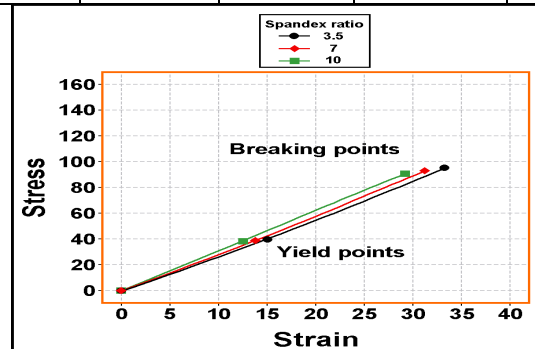
Fig. (10): Stress-strain curves of spandex/polyester woven fabrics as affected by spandex ratio.
