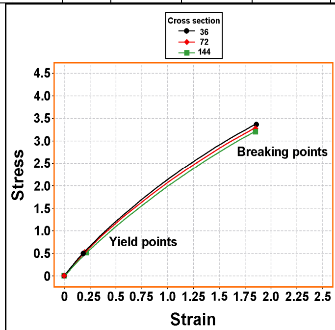
Fig. (2): Stress-strain curves of spandex/polyester spun yarn as affected by yarn cross section.
