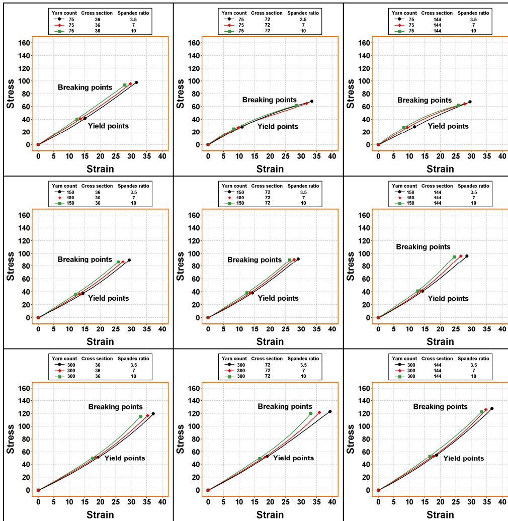
Fig. (7): Stress-strain curves of spandex/polyester woven fabrics as affected by the interaction effect among yarn count, cross section and spandex ratio.
