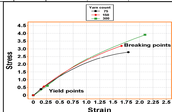
Fig. (1): Stress-strain curves of spandex/polyester spun yarn as affected by yarn count.
