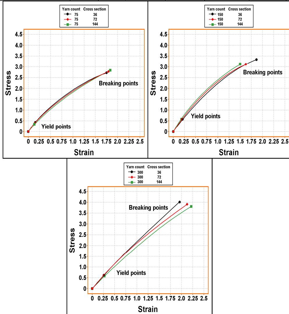
Fig. (4): Stress-strain curves of spandex/polyester spun yarn as affected by the interaction effect between yarn count and cross section.
