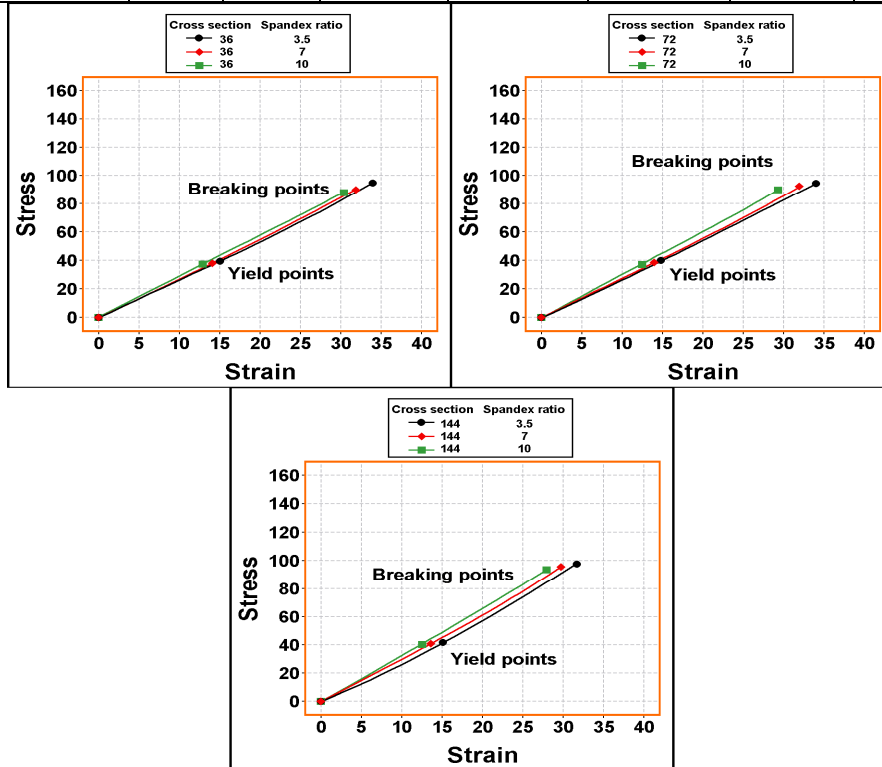
. (13): Stress-strain curves of spandex/polyester woven fabrics as affected by the interaction effect between cross section and spandex ratio.
