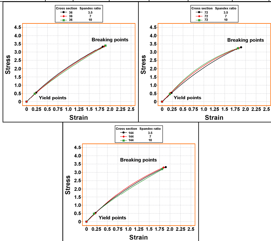
Fig. (6): Stress-strain curves of spandex/polyester spun yarn as affected by the interaction effect between cross section and spandex ratio
