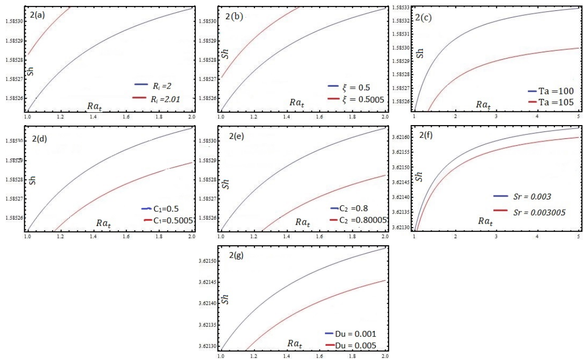
Fig. 2: Variability of Sh with Ra_t for different values of R_i , \xi , Ta , C_1 , C_2 , Sr , and Du respectively
