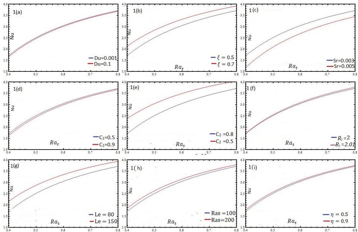
Fig. 1: Variability of Nu with Ra_t for different values of Du , \xi , Sr , C_1 , C_2 , R_i , Le , Ra_s , and \eta respectively
