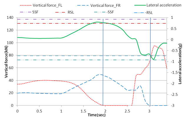
Fig. 11: Fishhook maneuver at 60 km/h on road bank 10%.
