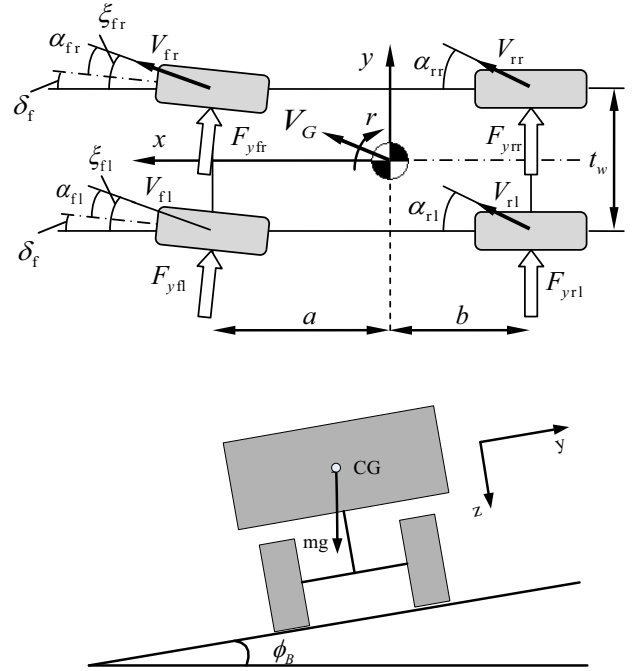
Fig. 1: A 2-DOF vehicle model with four wheels.
