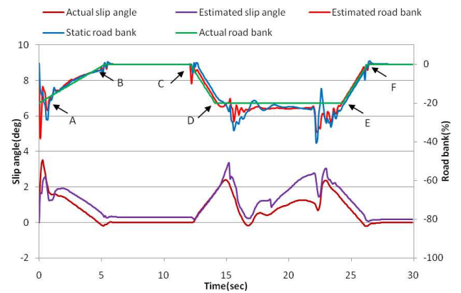
Fig. 6: Estimated results on low friction surface.
