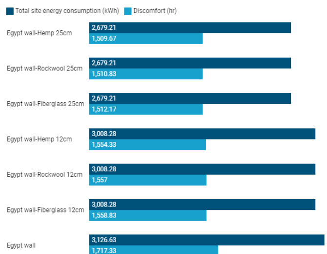
FIGURE 20. (RESULTS).
