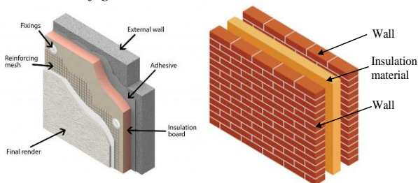
Figure 8. (Existing wall cross – section).
