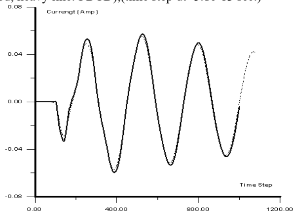
Fig. 11. f_k=5 GHz, \theta=45^\circ , other parameters as Fig. 10.
