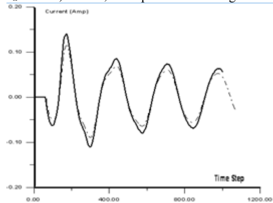
Fig.12. f_k=10 GHz, \theta=0^\circ , other parameters as Fig. 10.
