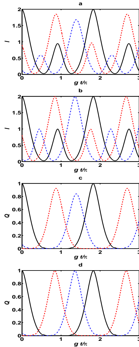
Fig. 2: Fock state field I(t) and \mathcal{Q}(t) for k_1 = k_2 = n_1 = n_2 = 5.0 , and r = 1.0 where (a,c) \delta = 0.6 , and (b,d) \delta = 0.001 for different T : T = 0.0 (black curve), T = 0.1 (dashed-dotted blue curve), T = 0.6 (dashed red curve).
