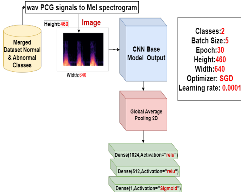
Fig. 2: The proposed approach architecture using Keras image CNN pre-trained models.
