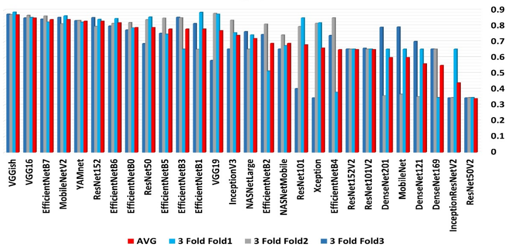
Fig. 14: The average validation accuracy for image and audio pre-trained CNN models utilizing three folds.
