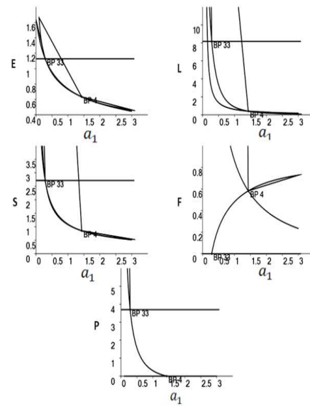
Fig. 14: We plot a bifurcation diagram for the system (9) with a_1 as bifurcation parameter for a higher predator saturation constant \beta_1 = 0.2 . In this case no Hopf bifurcation occurs.
