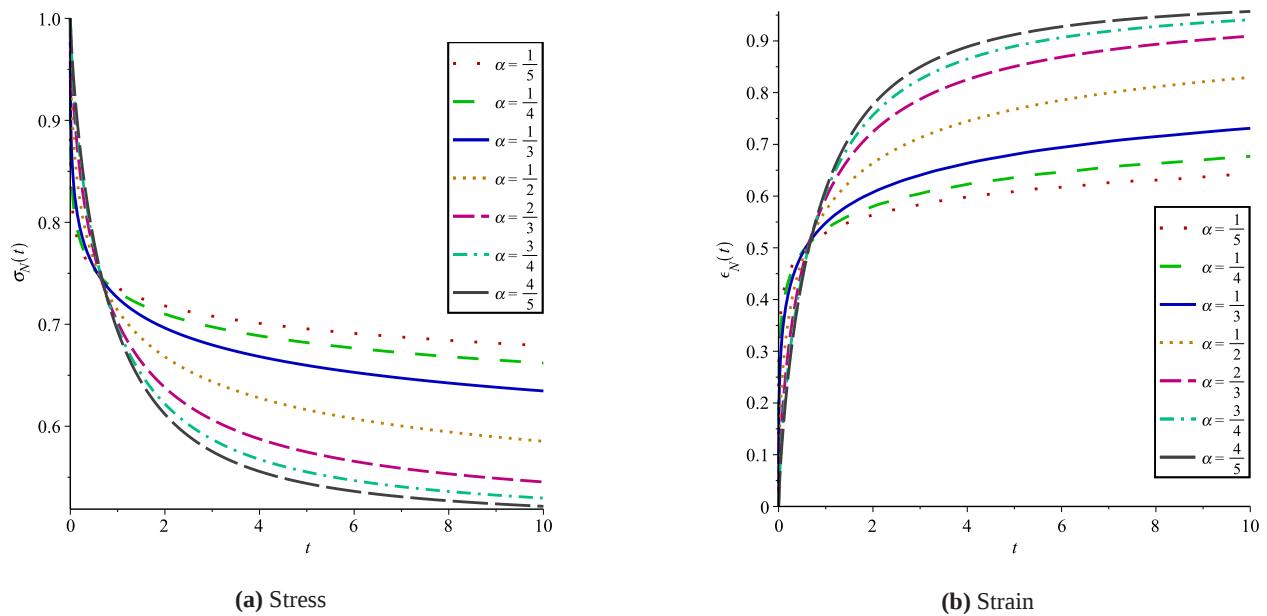
Fig. 1: The stress and strain functions of the model for different values of \alpha .
