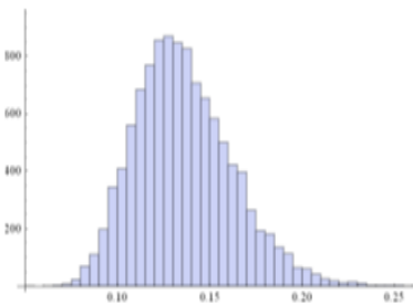
Fig. 4: Histogram of \alpha obtained by MCMC method.
