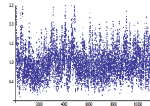
Fig. 2: Simulation number of \beta_1 obtained by MCMC method.
