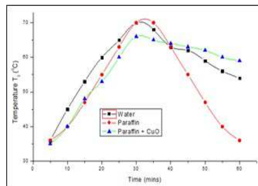
Fig. 6: Temperature distribution at section 3
