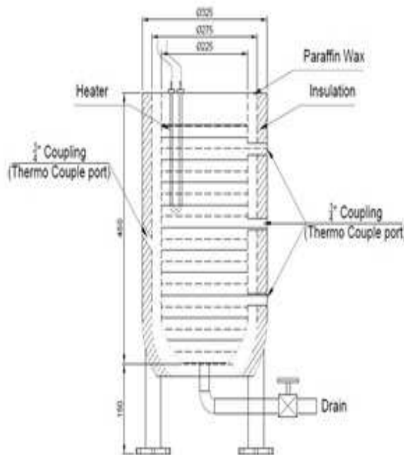
Fig. 2: Schematic layout
