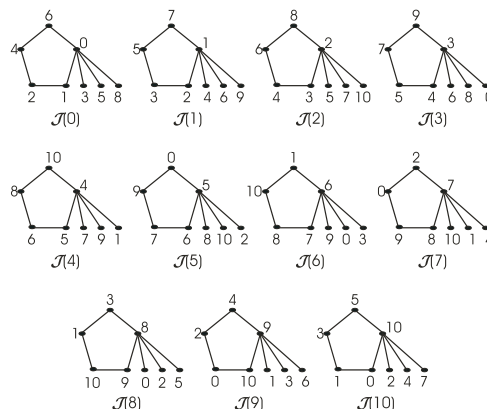
Fig. 3: C_5 \cup^v K_{1,3} -design for Cay(\mathbb{Z}_{11}, A = \mathbb{Z}_{11} \setminus \{0, 4, n-4\}) where v \in \mathbb{Z}_{11} .
