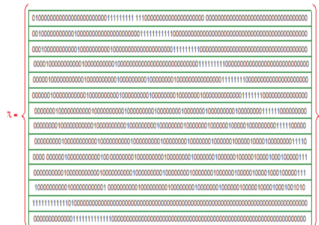
Fig. 8: Code \mathcal{R} induced from the graph design of example 6.
