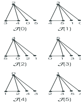
Fig. 6: C_3 \cup^v K_{1,2} -design for Cay(\mathbb{Z}_6, A = \mathbb{Z}_6 \setminus \{0\}) .
