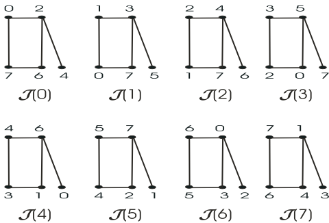
Fig. 2: C_4 \cup^v K_{1,1} -design for Cay(\mathbb{Z}_8, A = \mathbb{Z}_8 \setminus \{0, 3, n-3\}) where v \in \mathbb{Z}_8 .
