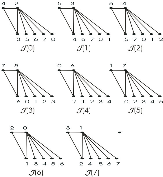
Fig. 1: C_3 \cup^v K_{1,4} -design for Cay(\mathbb{Z}_8, A = \mathbb{Z}_8 \setminus \{0\}) where v \in \mathbb{Z}_8 .
