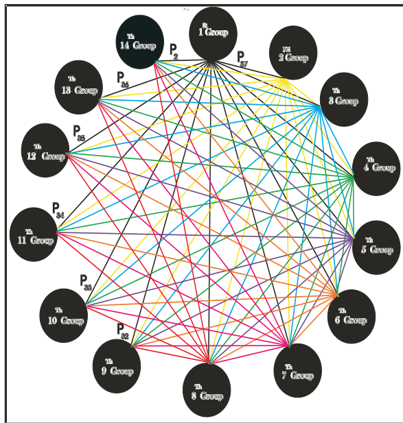
Fig. 7: Cay(\mathbb{Z}_{14}, A = \mathbb{Z}_{14} \setminus \{0\})
