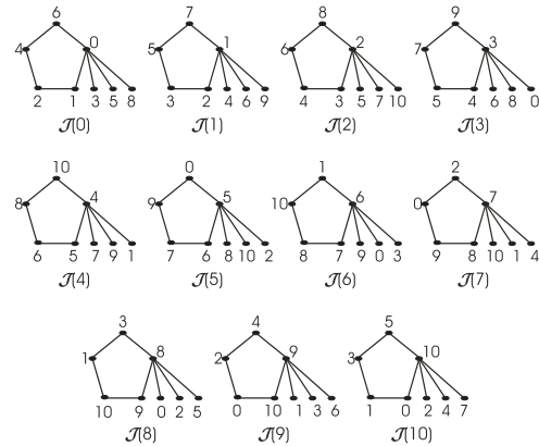
Fig. 3: C_5 \cup^v K_{1,3} -design for Cay(\mathbb{Z}_{11}, A = \mathbb{Z}_{11} \setminus \{0, 4, n-4\}) where v \in \mathbb{Z}_{11} .
