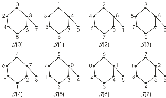
Fig. 4: C_6 \cup^v K_{1,1} -design for Cay(\mathbb{Z}_8, A = \mathbb{Z}_8 \setminus \{0\}) where v \in \mathbb{Z}_8 .
